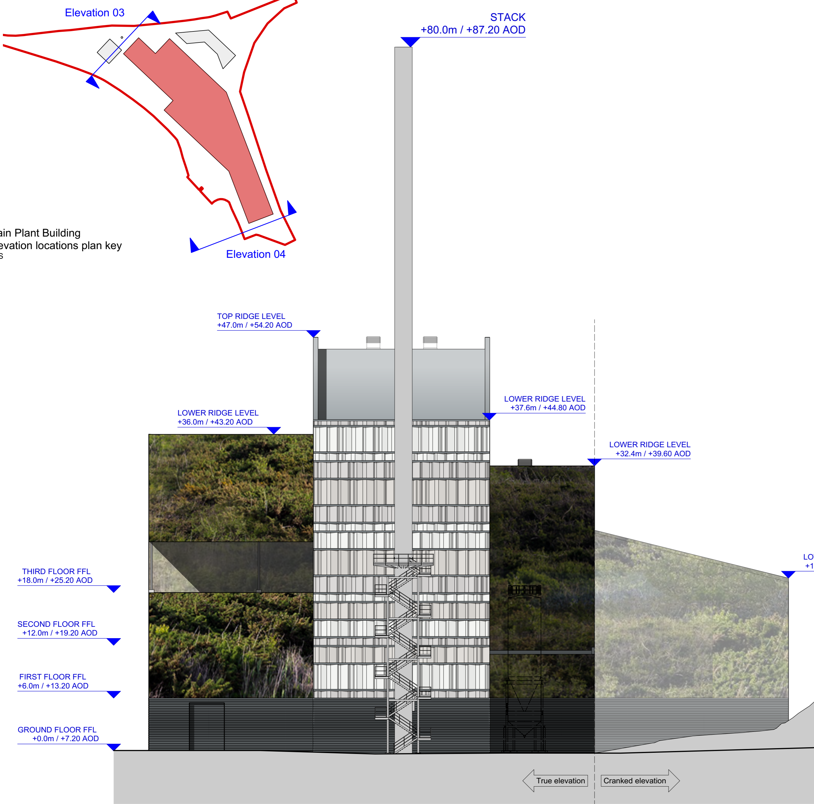
03 Elevation 03 (north-western) 1:250 @ A1 / 1:500 @ A3
