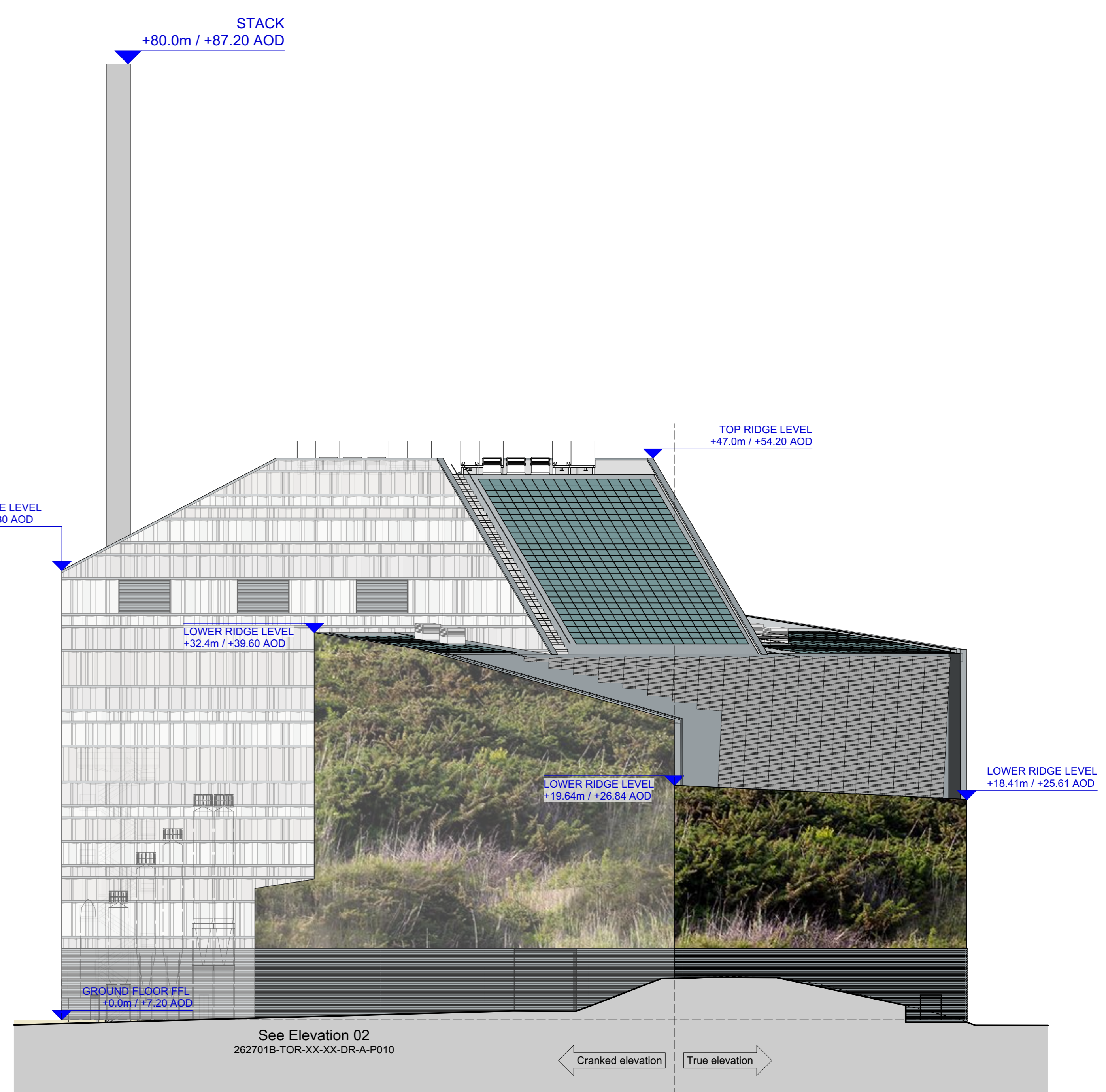
04 Elevation 04 (south-eastern) 1:250 @ A1 / 1:500 @ A3
